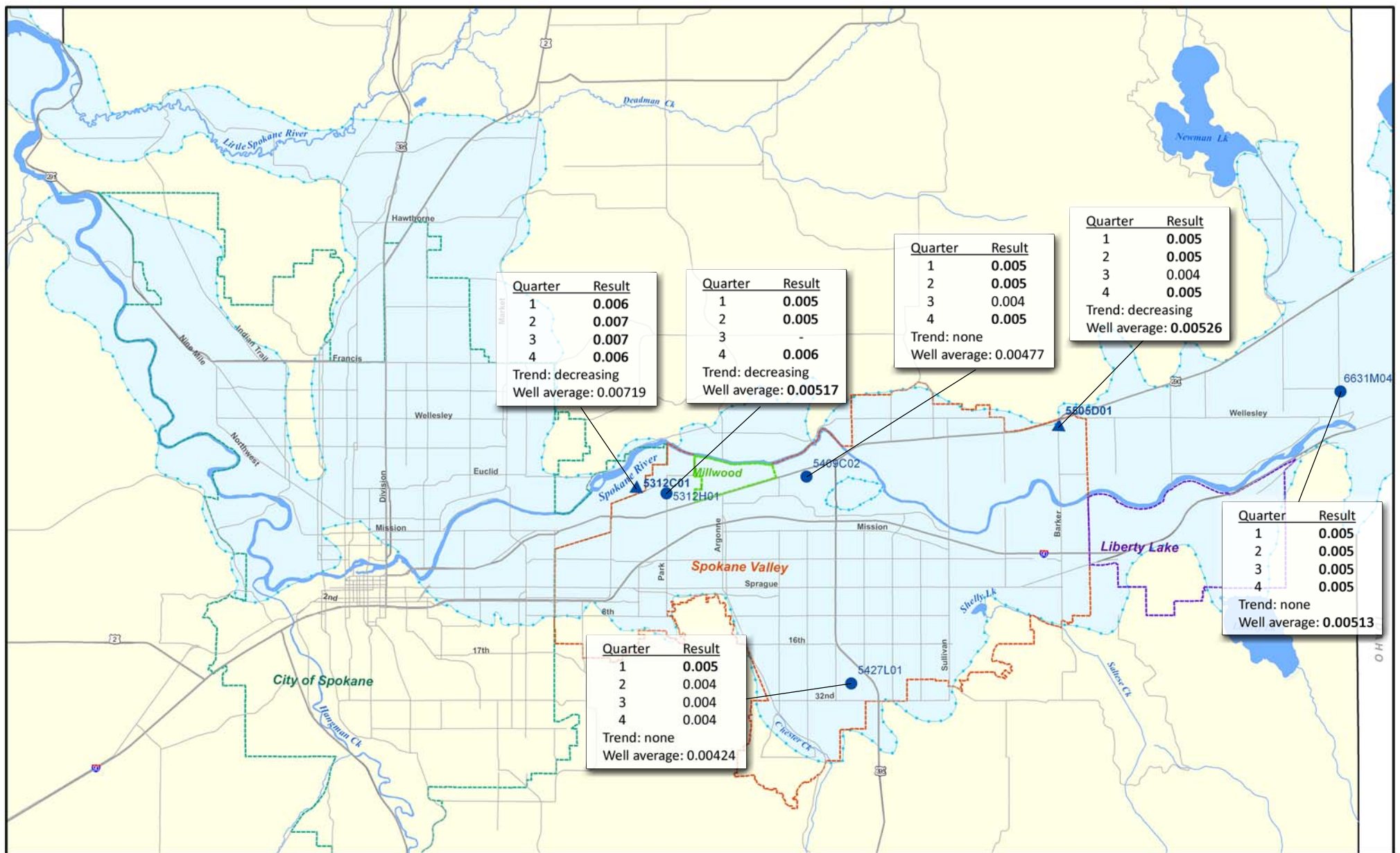
Figure 3 2007 Arsenic Results Exceeding Washington State Trigger Level
